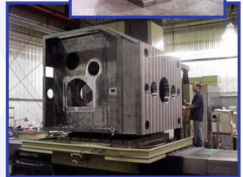
4 Axis Milling to 1,000 Cubic Feet
